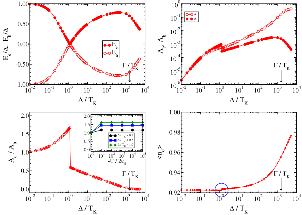
Figure 1. The NRG results on the Andreev states. The energies (a) and the corresponding spectral weights (b) of the subgap Andreev states for the U = \infty Anderson model. (c) The ratio A_e/A_h of the spectral weights of the Andreev states. Inset: A_e/A_h as a function of -U/2\epsilon_d . (d) Average occupation of the quantum dot level. \epsilon_d = -0.1D , U = \infty , \Gamma = 0.02D ( T_K \approx 3.88 \times 10^{-5} ).
