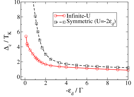
Figure 3. Phase diagram of the Anderson impurity model with superconducting leads (for \phi = 0 ) deduced from the NRG results. The phase boundaries for the infinite- U model (red solid line with circles) and for the particle–hole symmetric model (black dashed line with squares), respectively, have been calculated by the NRG method.
