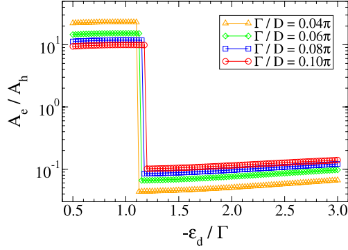
Figure 2. Results from the variational calculations. Plotted is the ratio A_e/A_h of the spectral weights as a function of -\epsilon_d/\Gamma for various values of \Gamma . \Delta/D = 0.1 .
