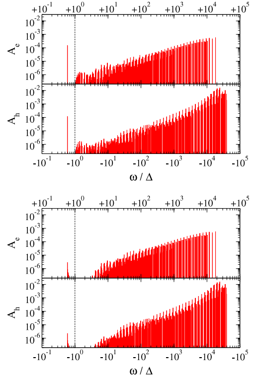
Figure 5. Raw data of the spectral weights of the discrete energy levels from the NRG calculation (a) at T = 0.1\Delta and (b) at T = 0.5 .
