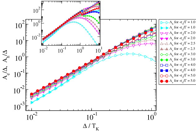
Figure 4. The NRG results of the spectral weights A_e ( A_h ) of the electron-like (hole-like) Andreev state as a function of \Delta/T_K at \epsilon_d = \phi = 0 for different values of \Gamma . Inset: the same in a wider range of \Delta/T_K including the doublet phase.
